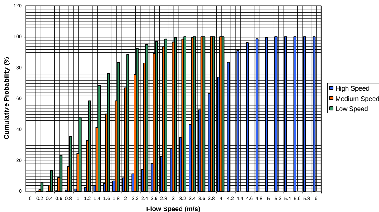
Figure 36 – Tidal Current Histogram (% Cumulative Probability)
