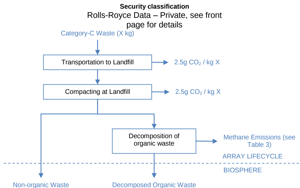
Figure 31 – Flowchart for modelling of Category-C waste disposal
