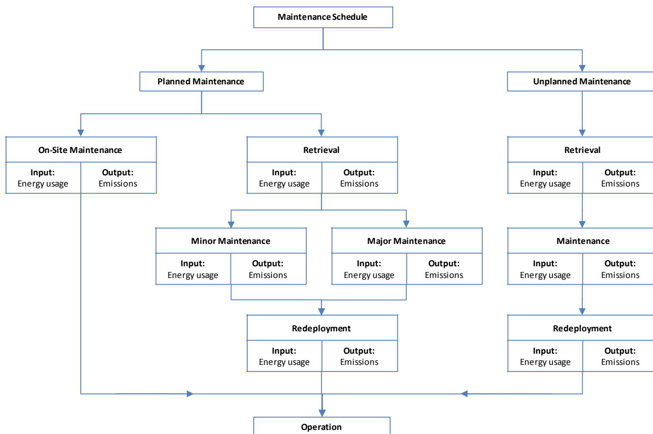
Figure 7 – Model of array life cycle – maintenance element
